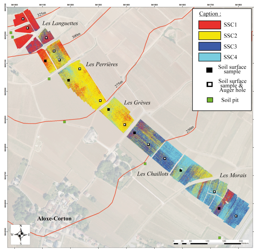
Figure 2. Distribution of four soil surface classes along the hillslope of Aloxe-Corton.
